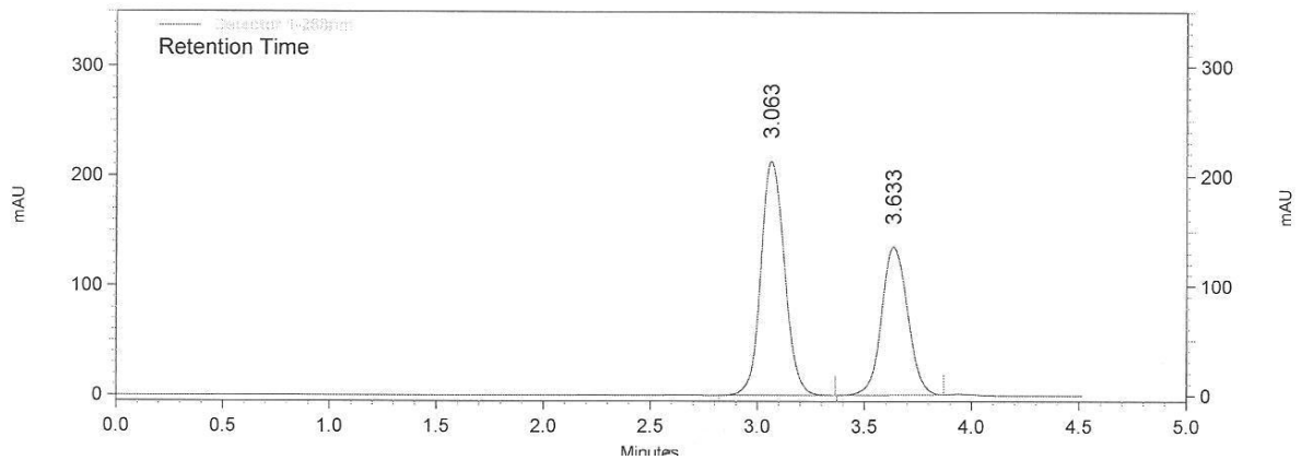
Figure 23: Chromatogram of robustness regarding wavelength 288nm
